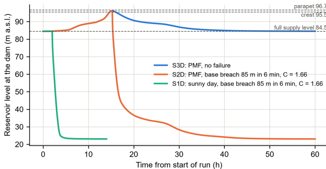
Figure 15 - Reservoir level at the dam, base runs.
