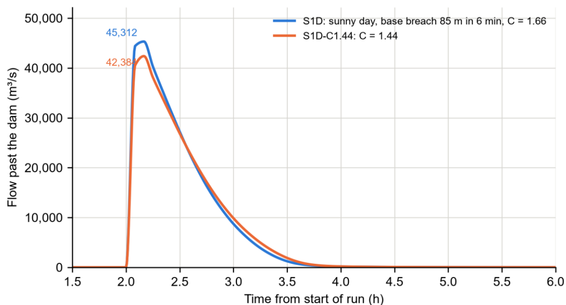
Figure 23 - Flow past the dam for the two breach weir coefficients, sunny day.
