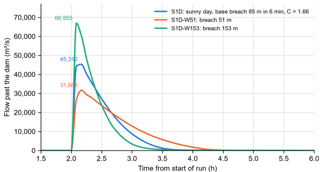
Figure 22 - Flow past the dam for the sunny-day breach-width runs (51, 85 and 153 m).
