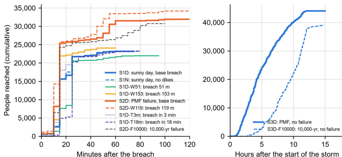
Figure 29 - People reached against time: failures from the breach (left), the PMF without failure from the start of the storm (right).
