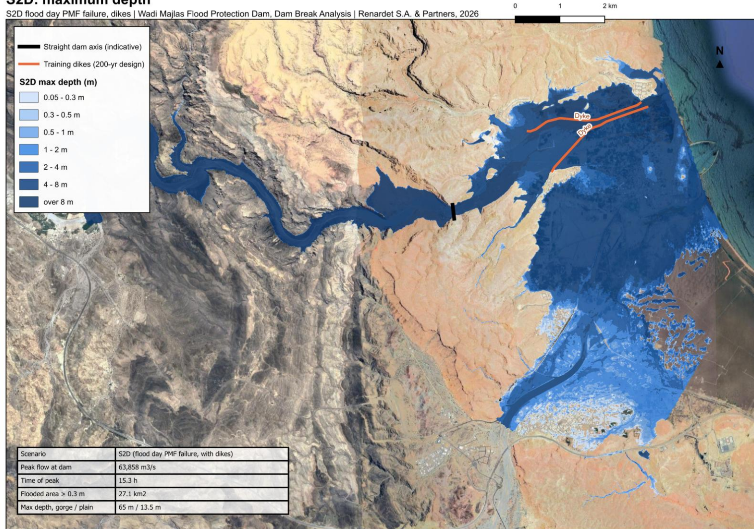
Figure 20 - S2D, flood-day (PMF) failure, dikes in place: maximum depth.
