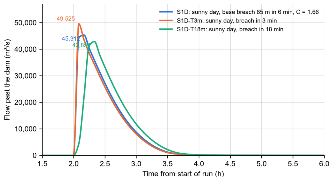
Figure 24 - Flow past the dam for the three formation times, sunny day (3, 6 and 18 min).
