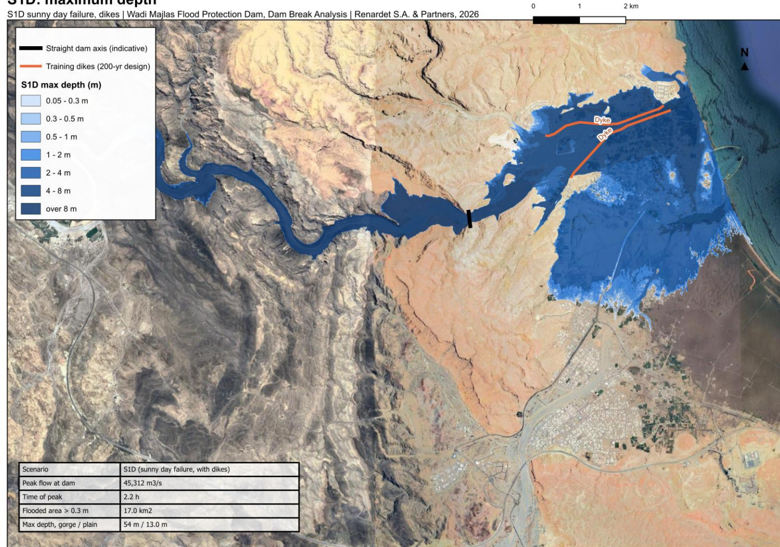
Figure 16 - S1D, sunny-day failure, dikes in place: maximum depth.
