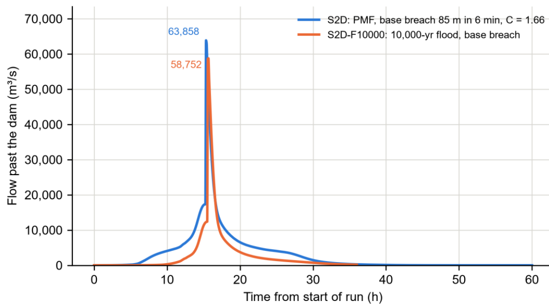
Figure 26 - Flow past the dam for the flood-day failure during the PMF and during the 10,000-year flood.
