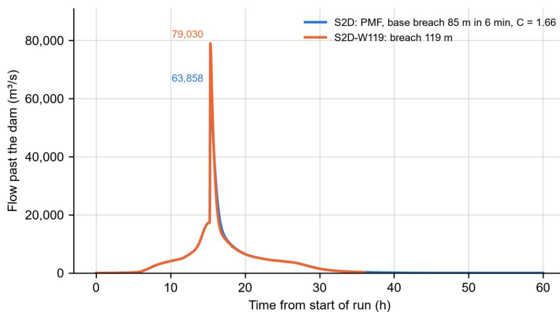
Figure 25 - Flow past the dam for the flood-day breach-width check (85 and 119 m).
