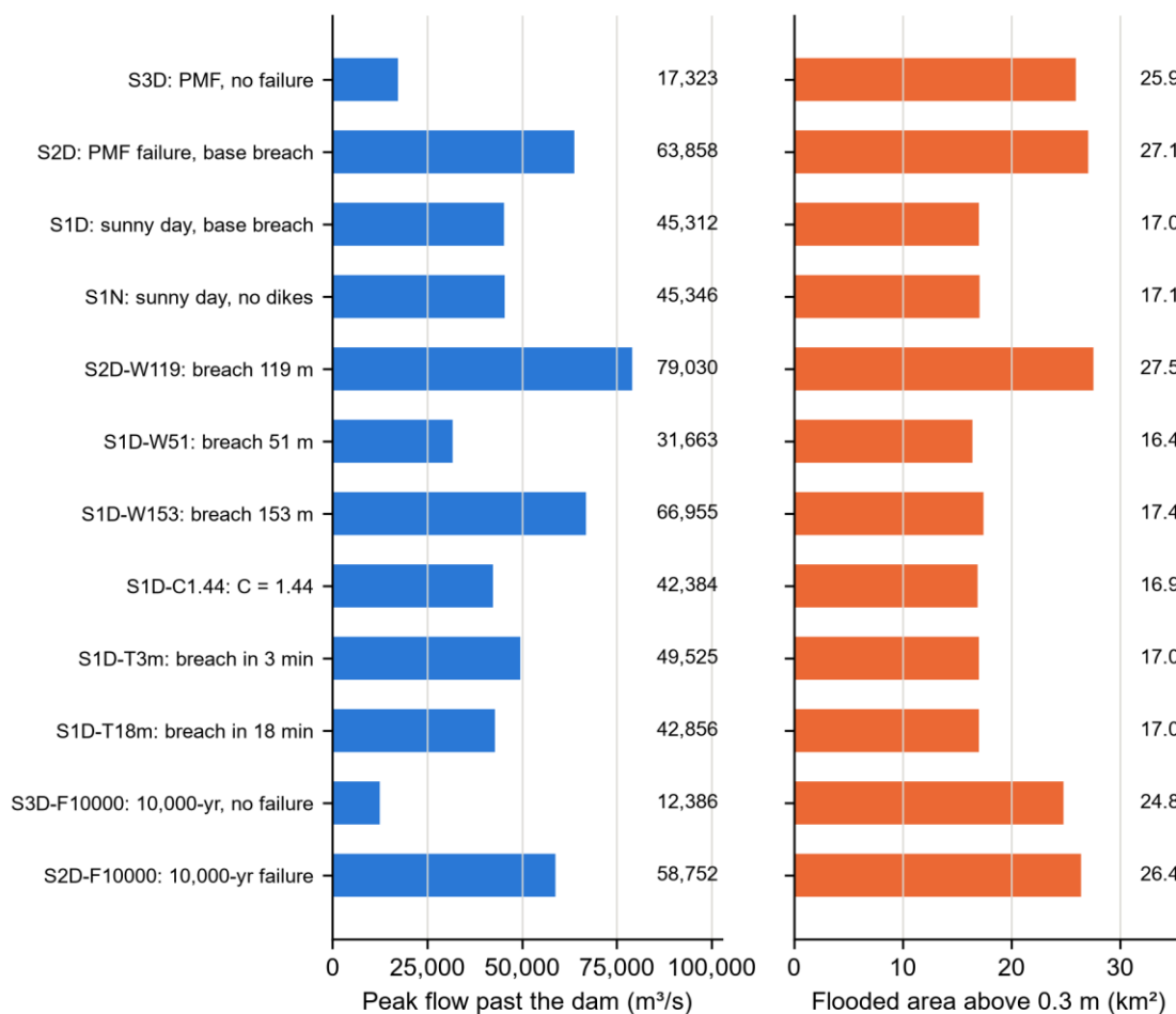
Figure 27 - Peak flow and flooded area of all runs.
