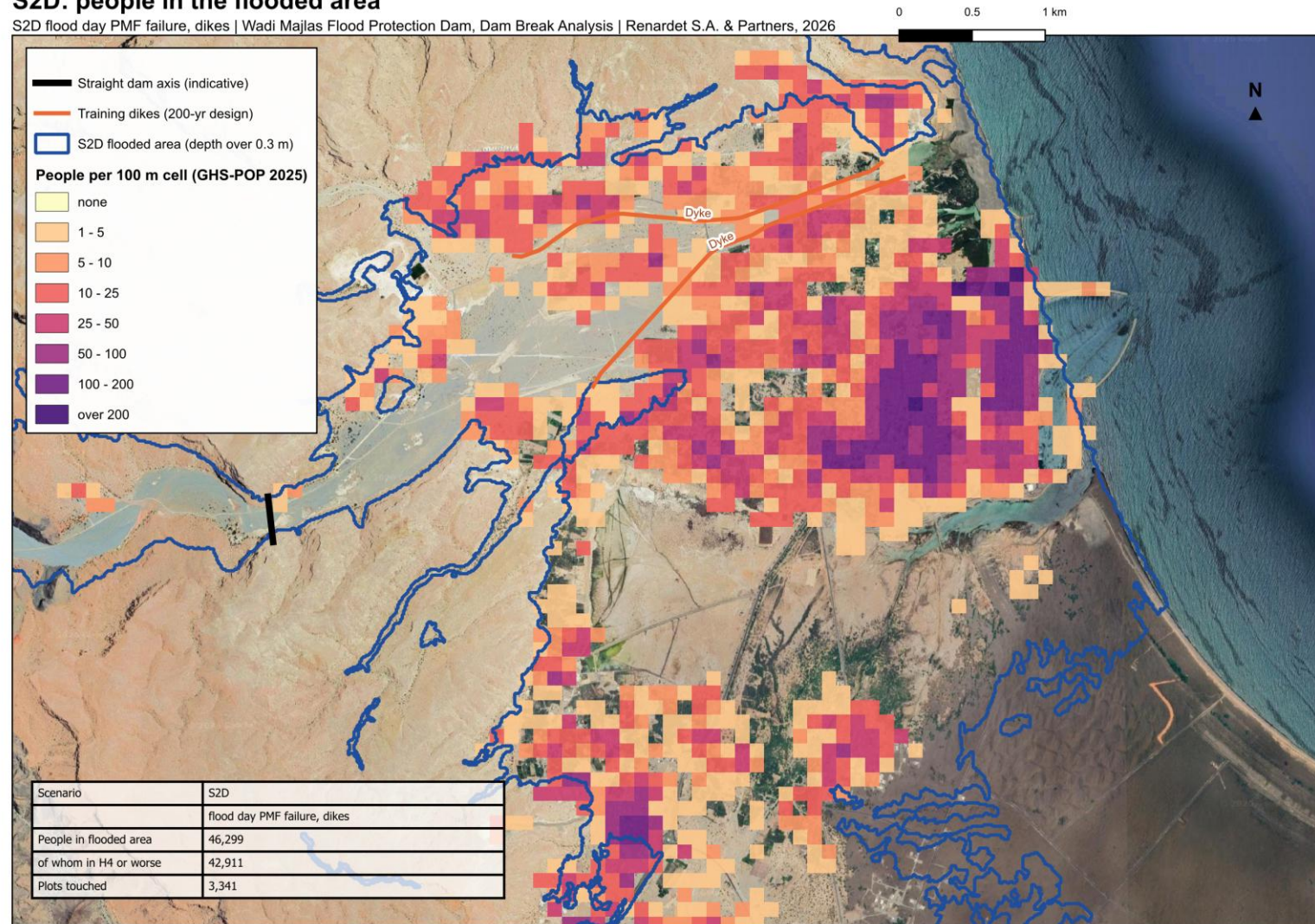
Figure 31 - S2D: people per 100 m cell (GHS-POP 2025) with the flooded area outlined.
