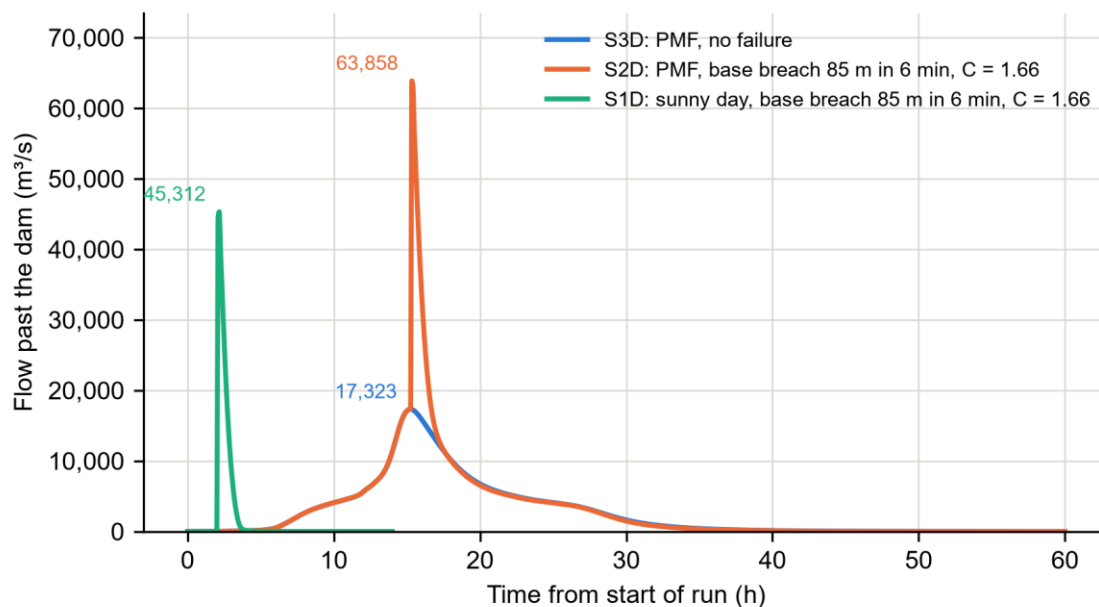
Figure 14 - Flow past the dam, base runs with dikes.
